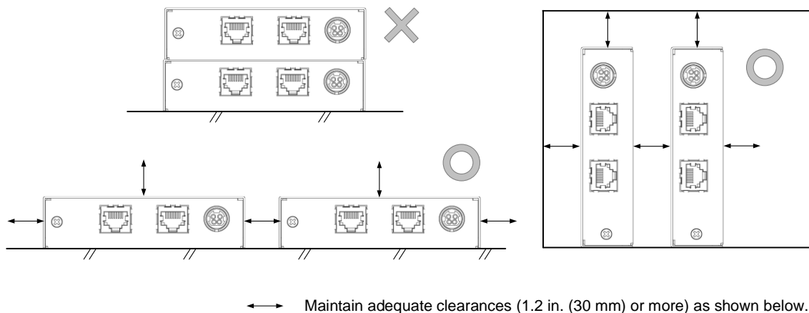
[Fig. 6.1] Necessary clearances
