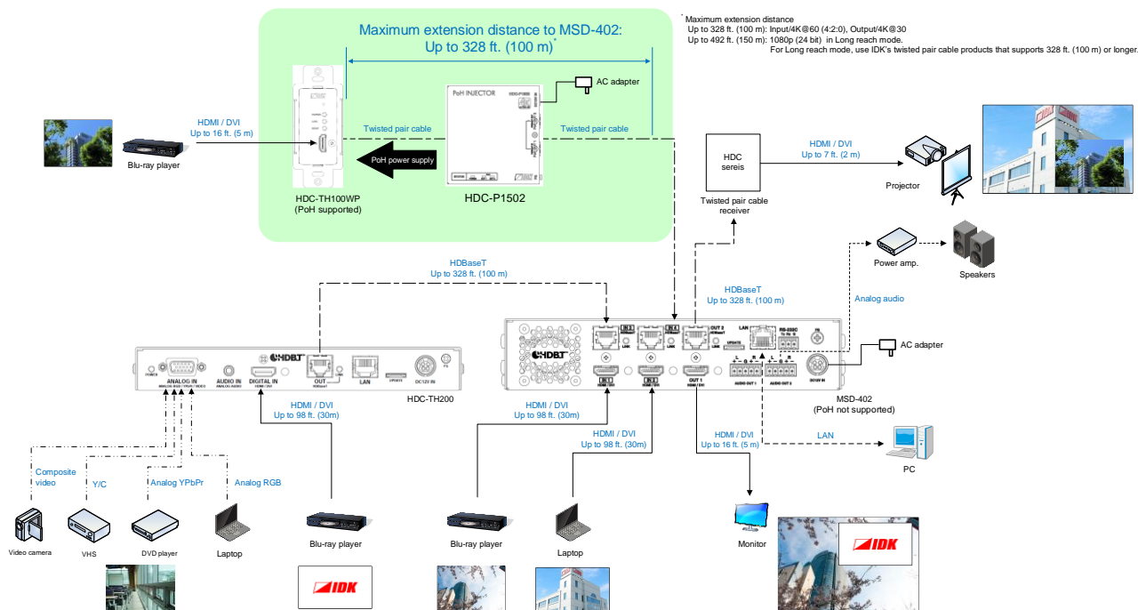
[Fig. 5.1] Application example (HDC-TH100WP and MSD-402 are connected)
